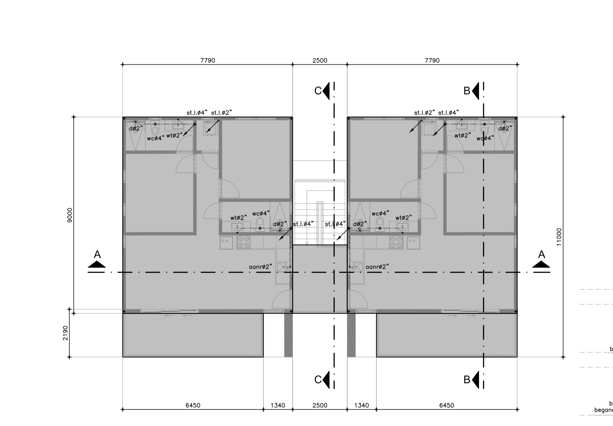
RIOLERINGSPLAN VERDIEPING APPARTEMENT TYPE B
