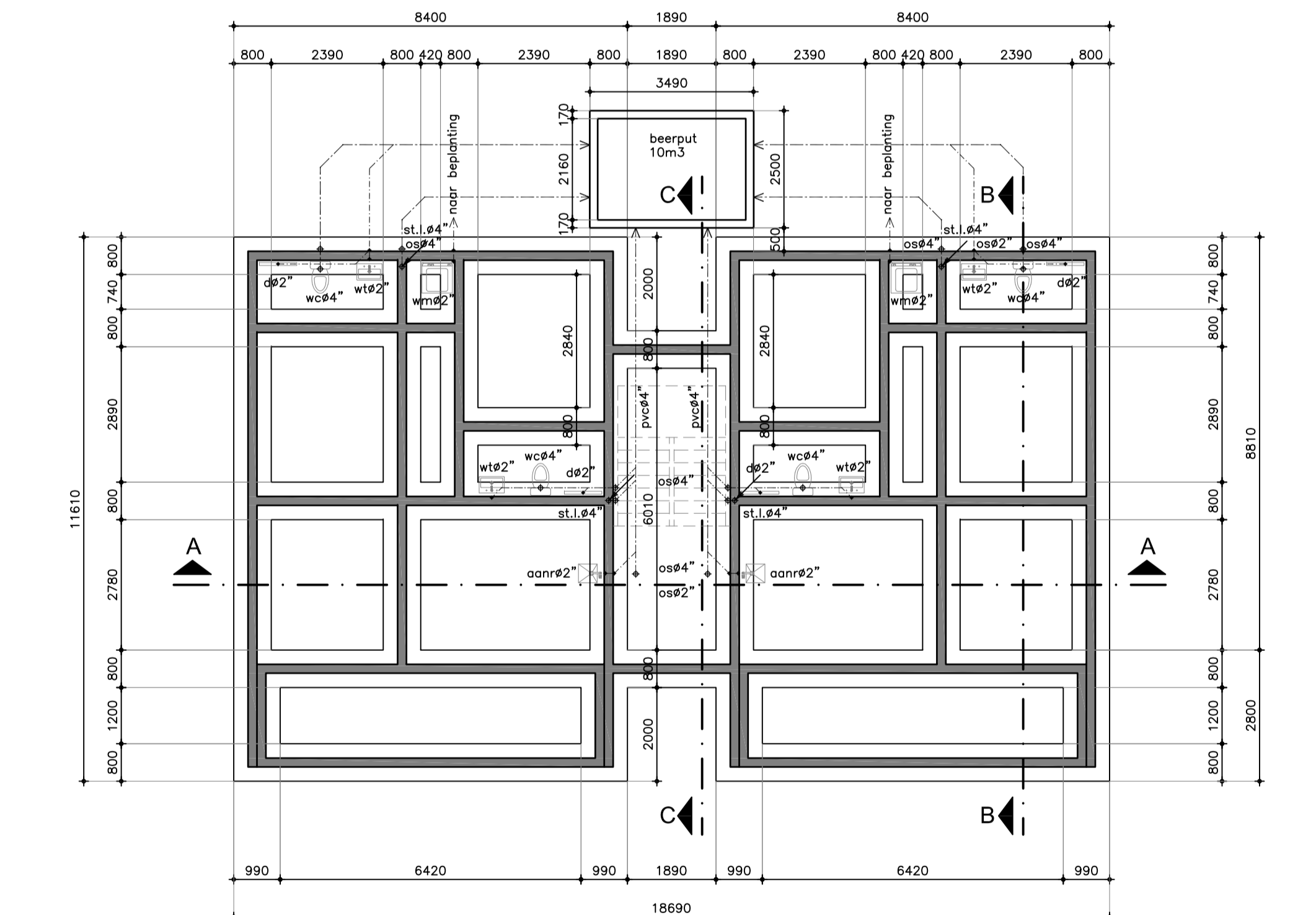
FUNDERINGS- RIOLERINGSPLAN BEGANE GROND APPARTEMENT TYPE B
